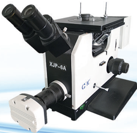
Metallographic microscope
